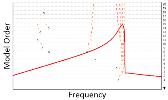
Wrong results in a stabilization diagram based on linear assumptions
