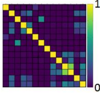
The MAC matrix shows high correlation between numerical and experimental mode shapes
